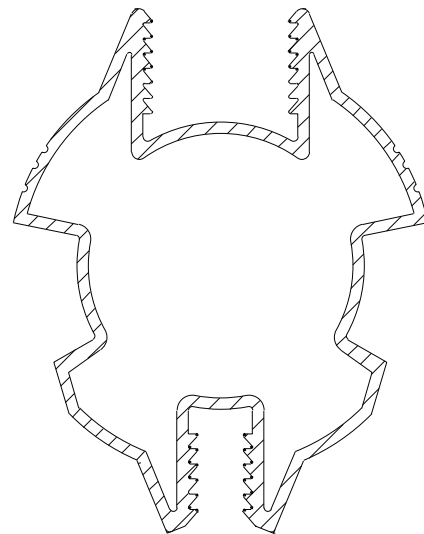
135°-160° Aluminium Art. No. 206760
