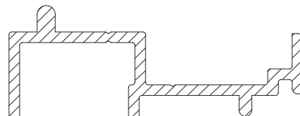
French Door Spacer Art. No. 200367
