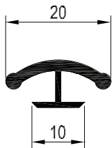
Inside Bay Cover Profile White Art. No. 240143 Laminated Art. No. 240133
