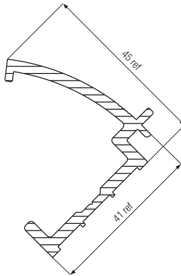
120°-135° Aluminium Art. No. 240103
