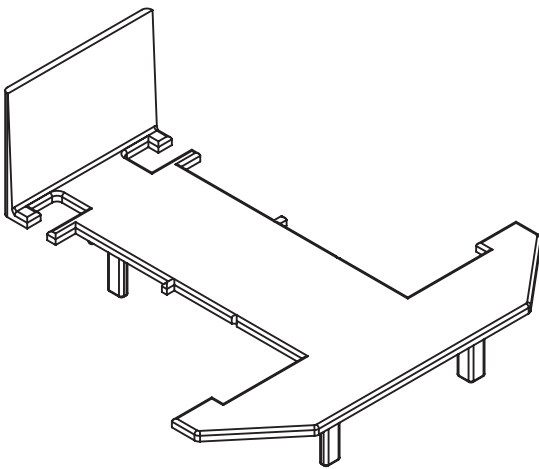
Dummy Mullion End Cap for Low Threshold For REHAU TOTAL70c Transom / Mullion (546085) Art. No. 200111
