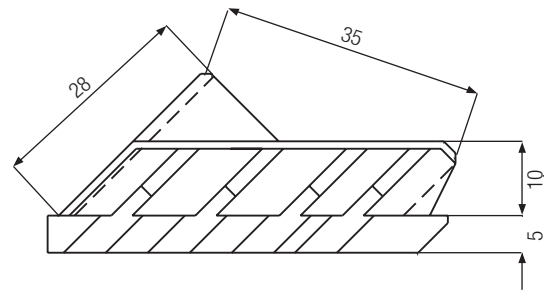
Weldable Corner Joint for Door Sash T and Z Art. No. 259036
