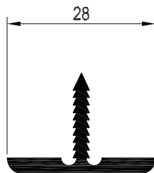
Inside Cover Profile White Art. No. 558170 Laminated Art. No. 576530
