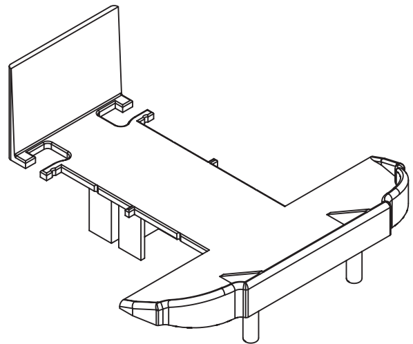
Dummy Mullion End Cap for Low Threshold For REHAU TOTAL70s Transom / Mullion (546665) Art. No. 286934
