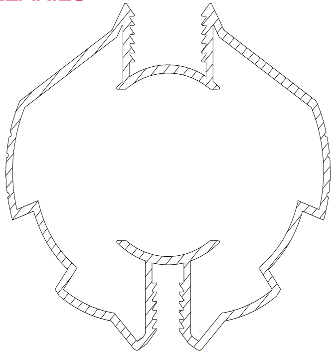
100°-120° Aluminium Art. No. 206780
